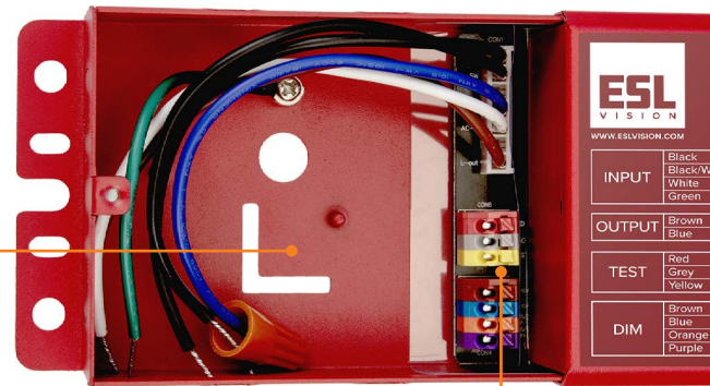
Fast Installation with Push Pin Connectors
