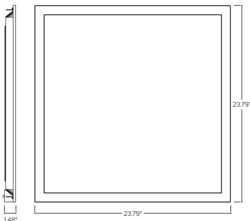
2x2 ESL-CSS-822-22-2030W-3550K
