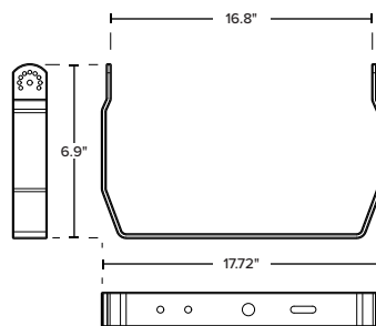
Yoke Mount
