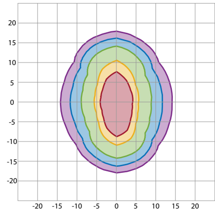
Isocandela Diagram
