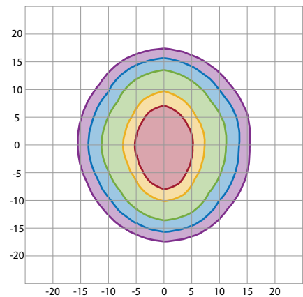
Isocandela Diagram
